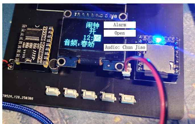
Figure 4. System realization in kind
