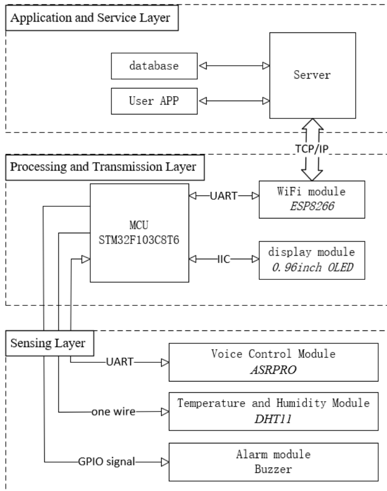
Figure 1. Block diagram of hardware structure design
