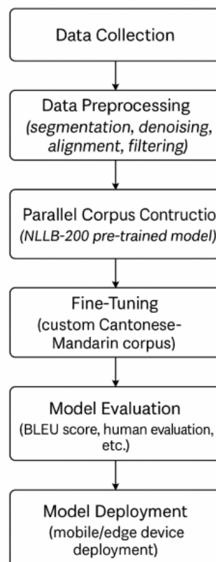
Figure 1. Workflow of Cantonese-Mandarin translation using the NLLB-200 model
