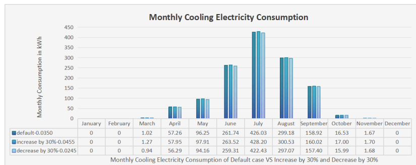
Figure 11. Monthly cooling electricity consumption of default case vs increase case and decrease case
