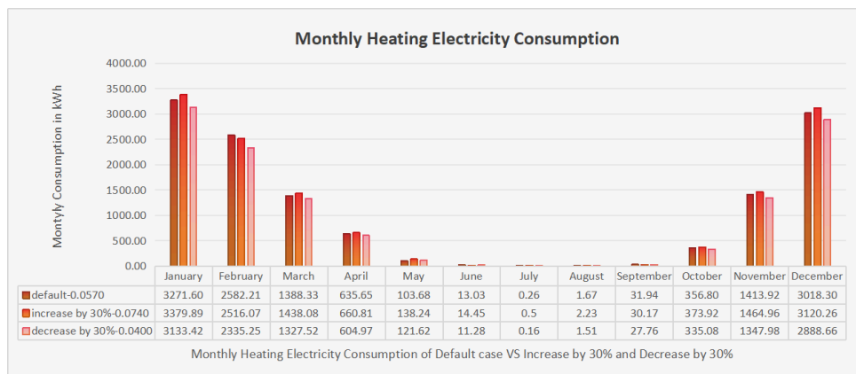
Figure 7. Monthly heating electricity consumption of default case vs increase case and decrease case
