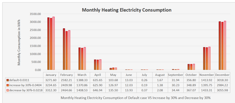
Figure 16. Monthly heating electricity consumption of default case vs increase case and decrease case
